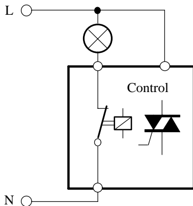
Figure 4. Three-wire circuit
