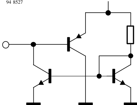
Figure 11. Tuner AGC – output (Pin 11)
