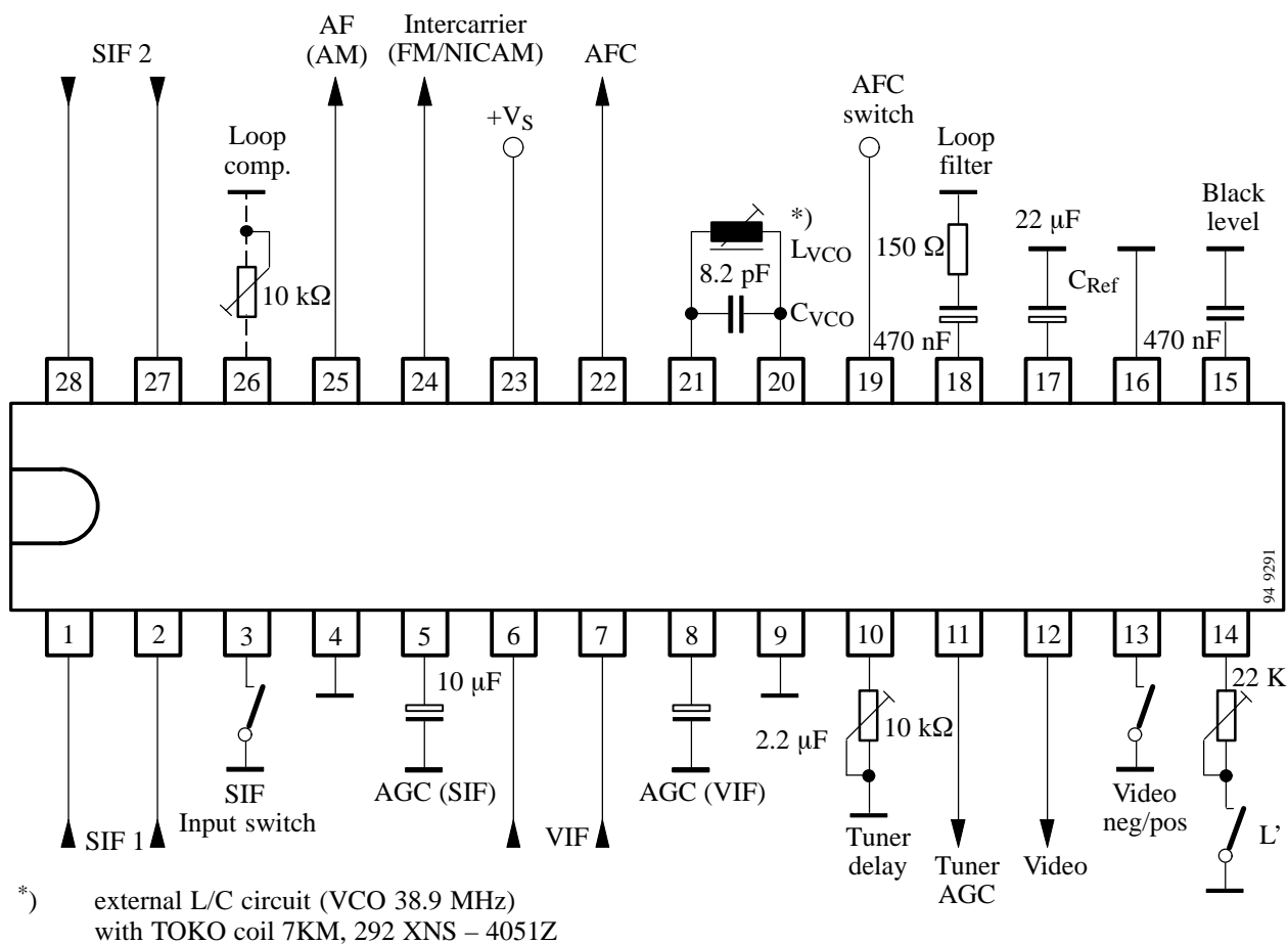
Figure 3. Test circuit
