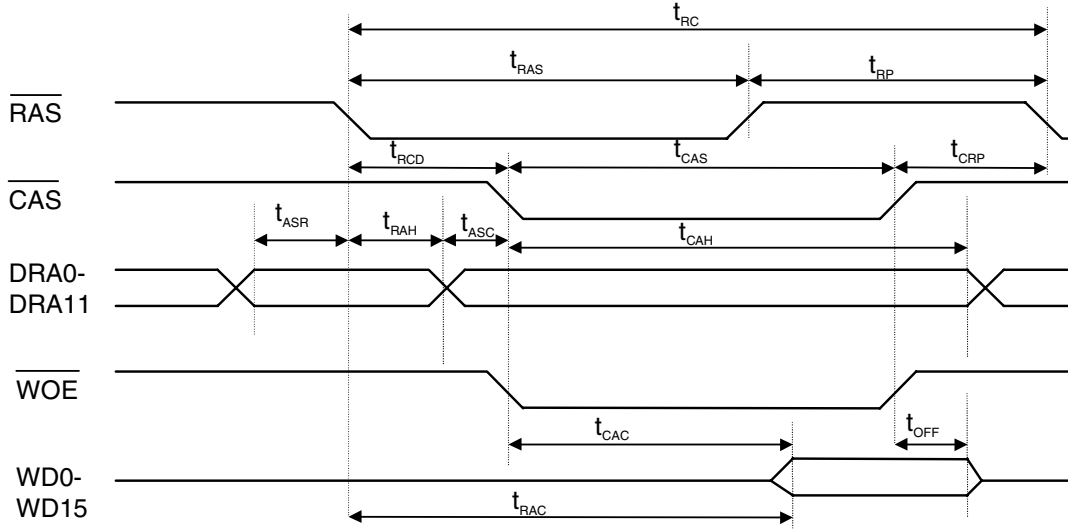
Figure 7. External DRAM Read Cycle
