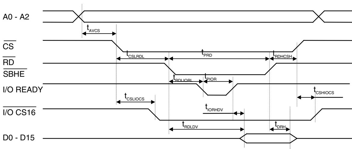
Figure 5. PC Host Interface Timing Diagram
