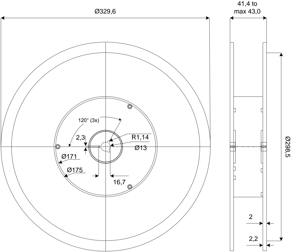
Figure 30. Shipping Reel
