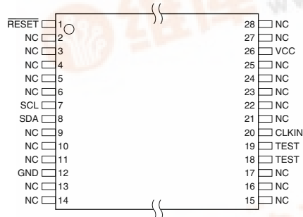
28-lead TSSOP
