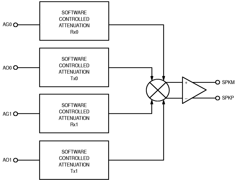
Figure 12. Speaker Mixer
