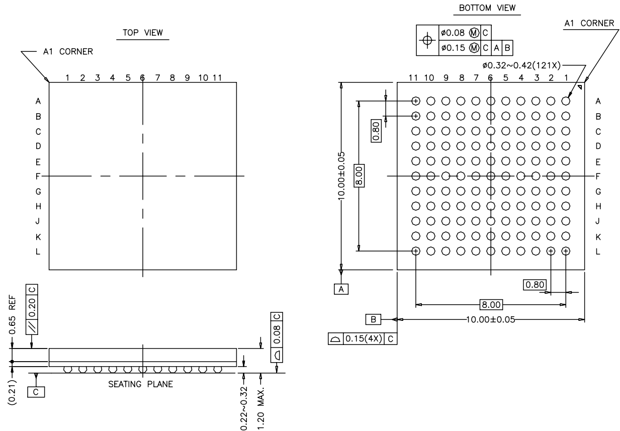
Figure 4. AT91FR4042 Package
