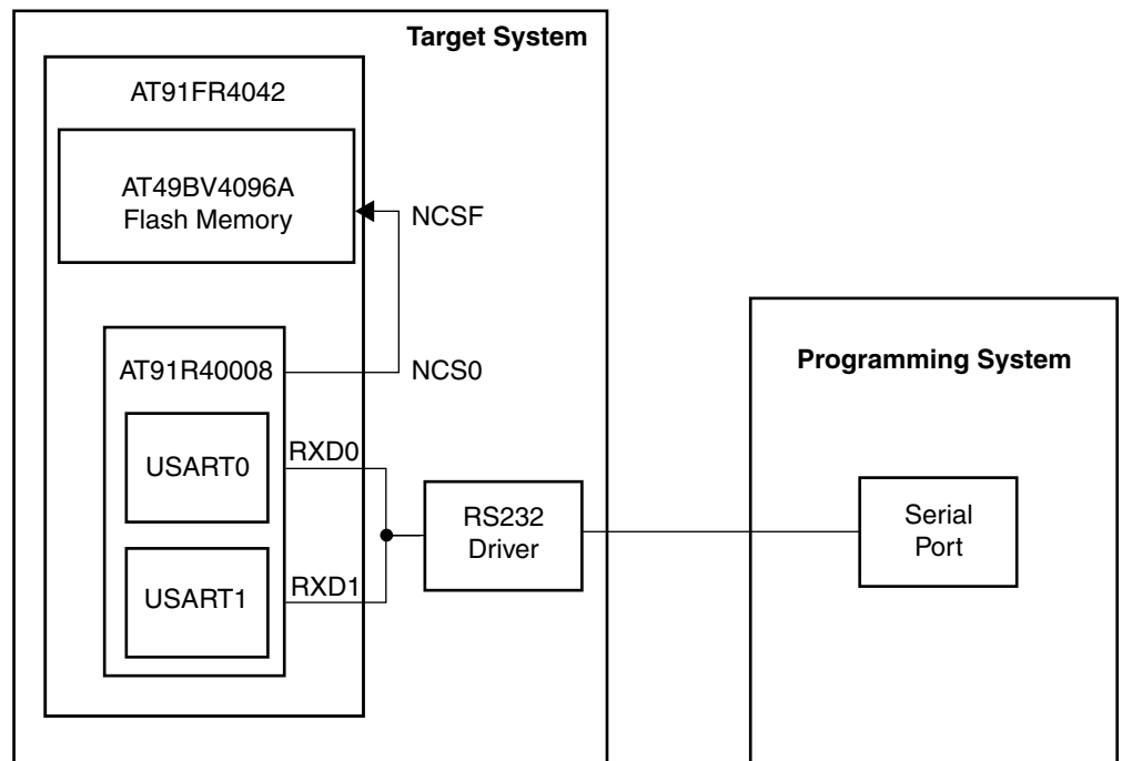
Figure 3. Flash Uploader
