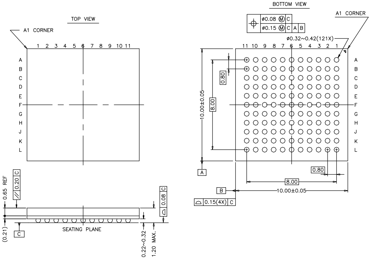
Figure 4. AT91FR40162 Package
