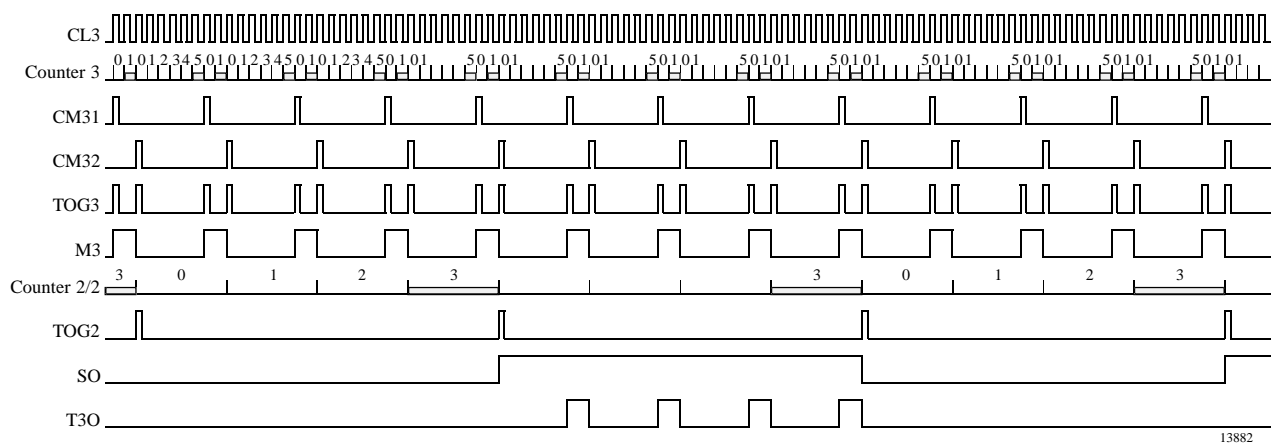
Figure 84. Burst modulation 2
