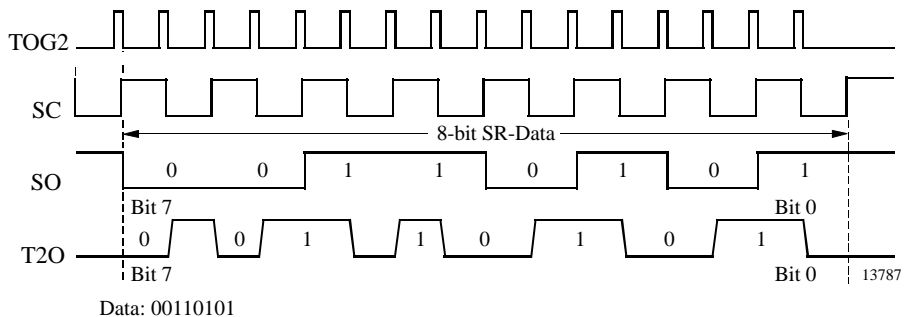
Figure 41. Manchester modulation
