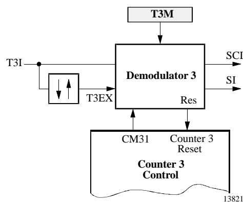
Figure 57. Timer 3 demodulator 3
