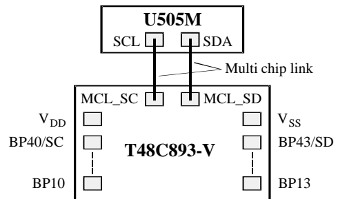
Figure 66. Multi-chip link
