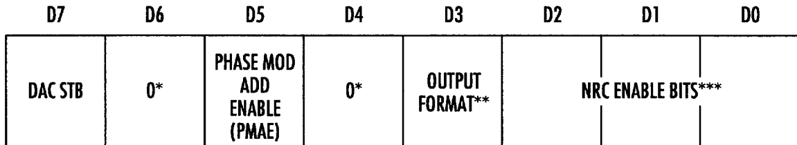
Figure 6. Asynchronous Mode Control (AMC) Register
