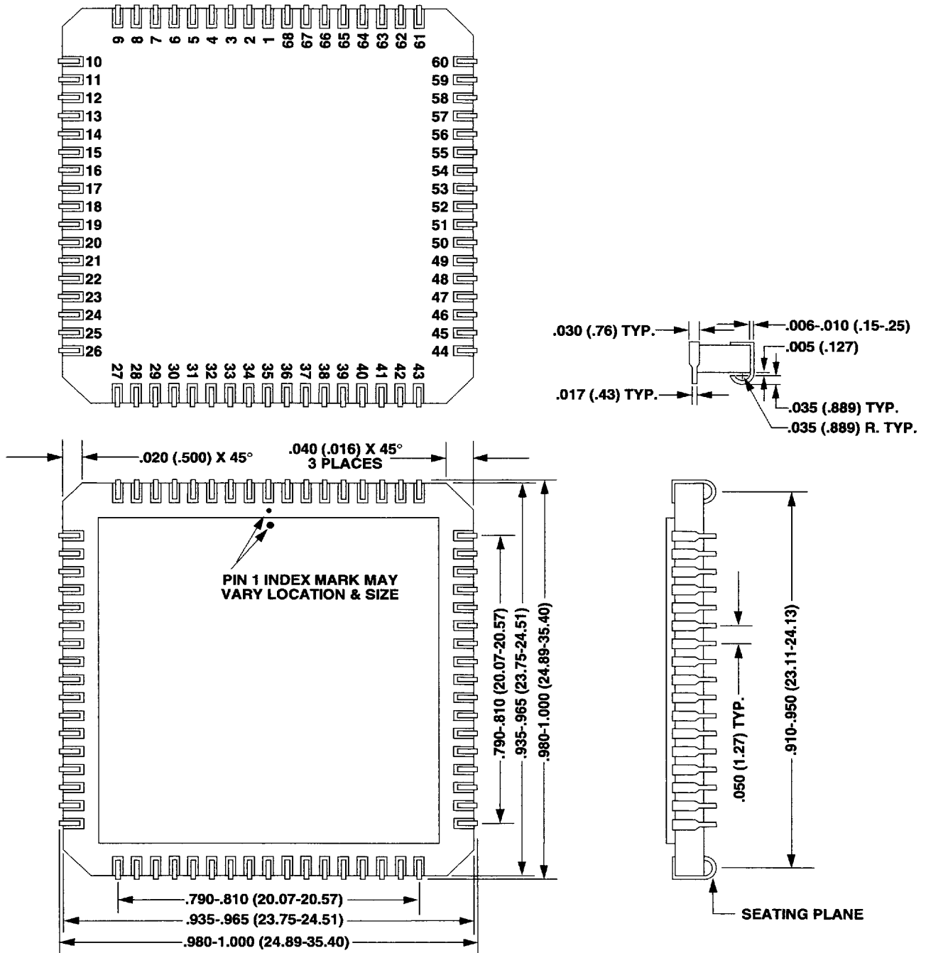
Figure 16. CLDCC Packaging
