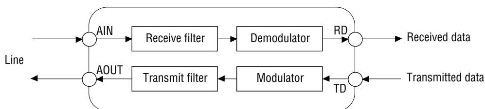
Figure 7 Signal Flow in Normal Operation
