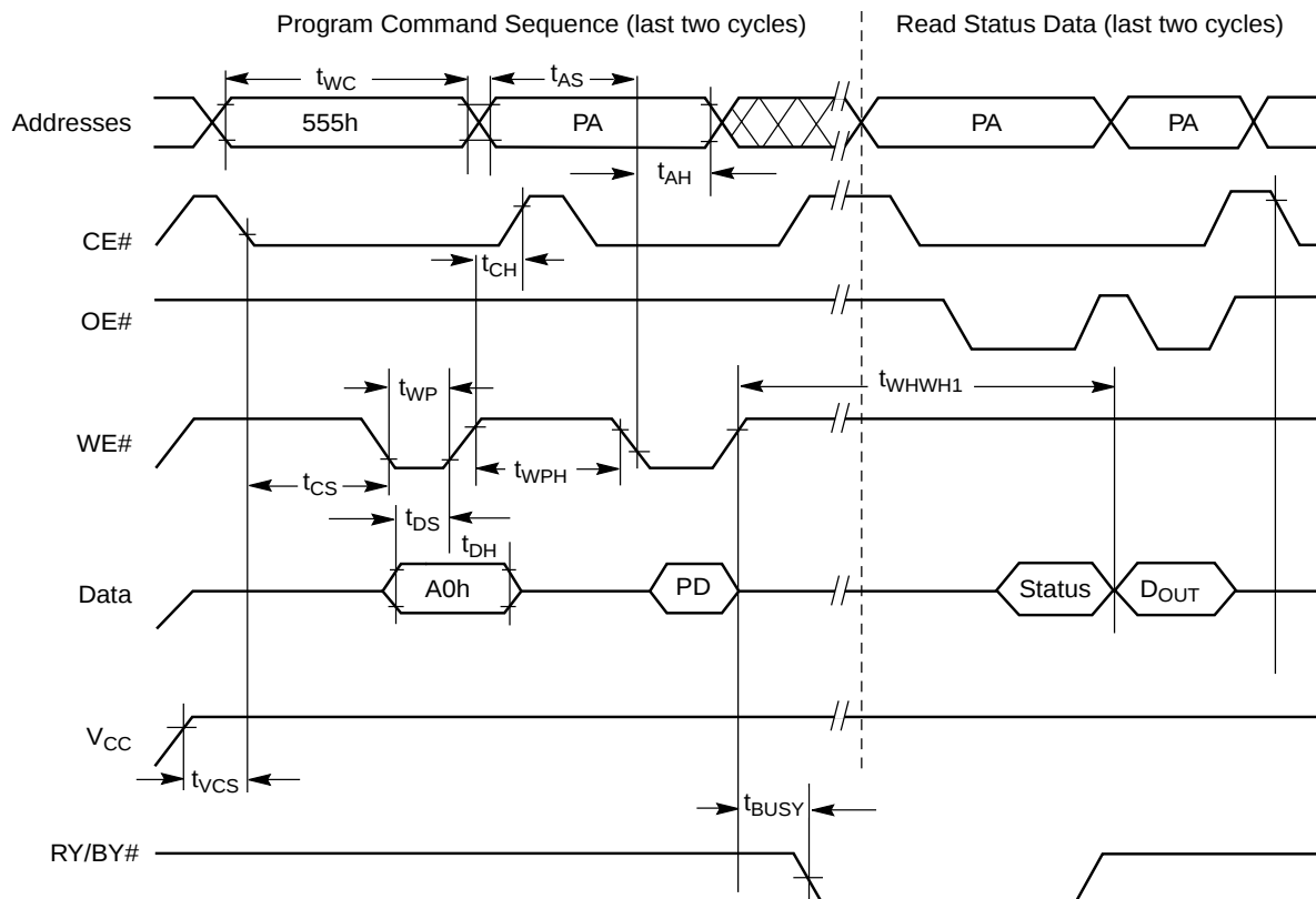
Figure 16. Program Operation Timings
