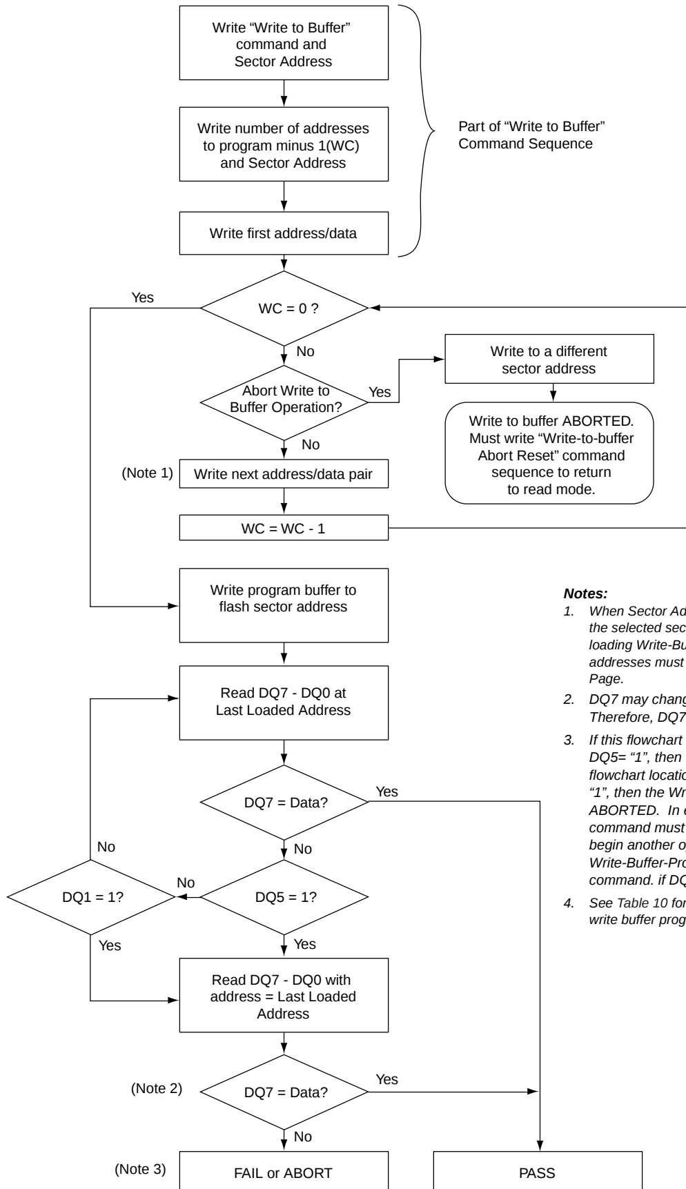
Figure 3. Write Buffer Programming Operation
