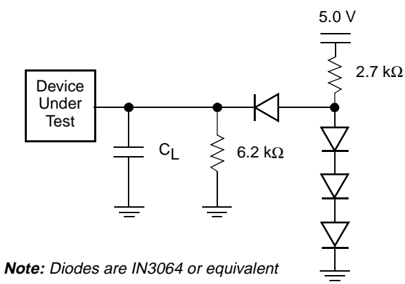
Figure 9. Test Setup
