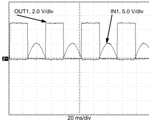
Figure 4. Low-Side Clamp
