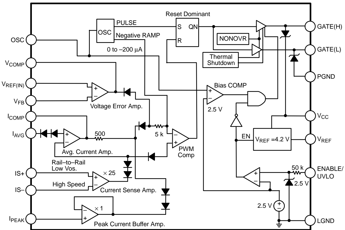
Figure 2. Block Diagram
