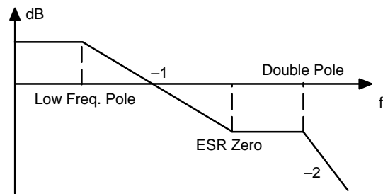
Figure 6. Bode Plot
