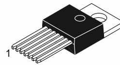
TO-220 SEVEN LEAD T SUFFIX CASE 821E
