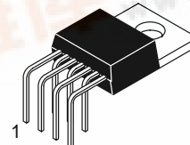
TO-220 SEVEN LEAD THA SUFFIX CASE 821H
