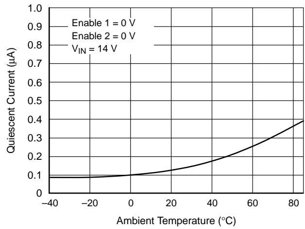
Figure 9. Quiescent Current
