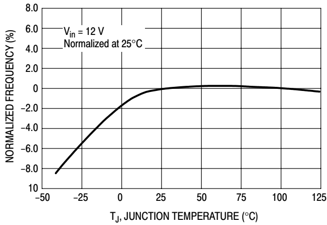
Figure 8. Oscillator Frequency
