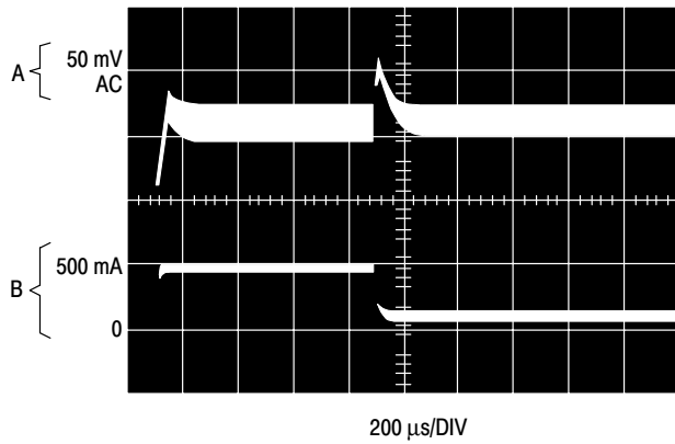
A: Output Voltage, 50 mV/DIV, AC Coupled B: 100 mA to 500 mA Load Pulse Figure 14. 500 mA Load Transient Response for Continuous Mode Operation, L = 330 \mu\text{H} , C_{\text{out}} = 300 \mu\text{F}
