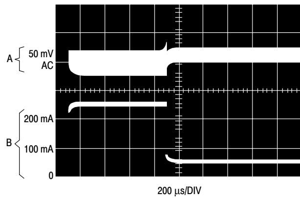
A: Output Voltage, 50 mV/DIV, AC Coupled B: 50 mA to 250 mA Load Pulse Figure 15. 250 mA Load Transient Response for Discontinuous Mode Operation, L = 68 \mu\text{H} , C_{\text{out}} = 470 \mu\text{F}
