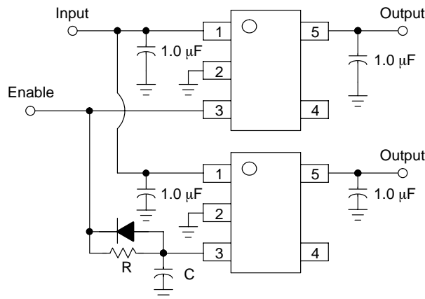
Figure 20. Delayed Turn-on
