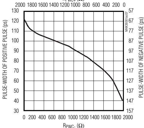
PULSE WIDTH vs. R_{PWC}
