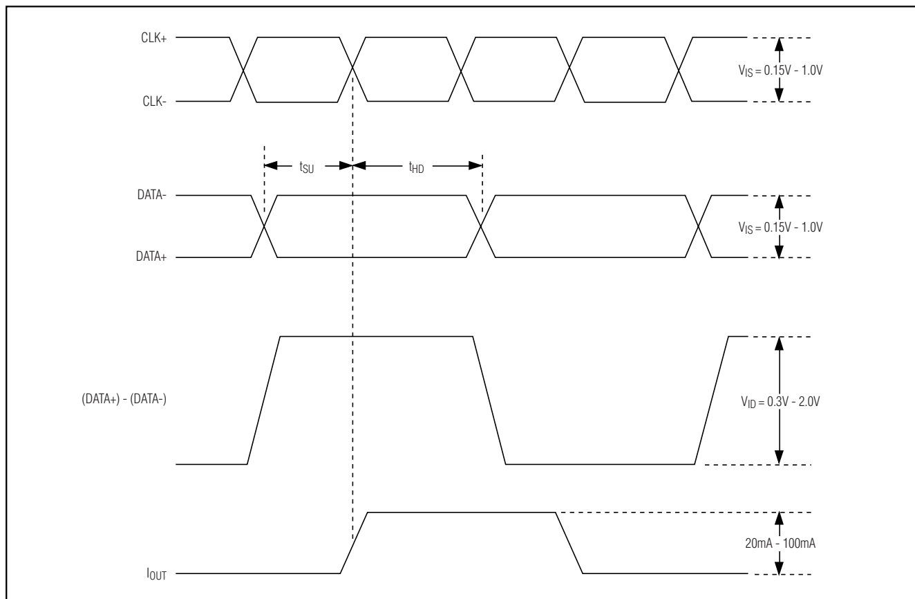
Figure 2. Required Input Signal, Setup/Hold Time Definition, and Output Polarity
