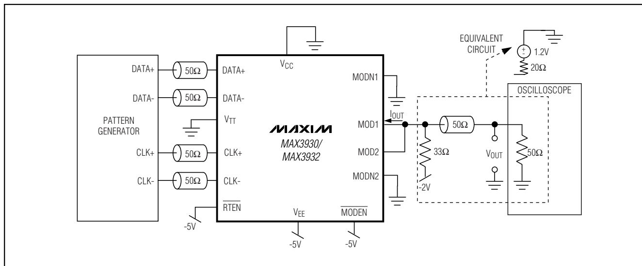
Figure 1. Test Circuit
