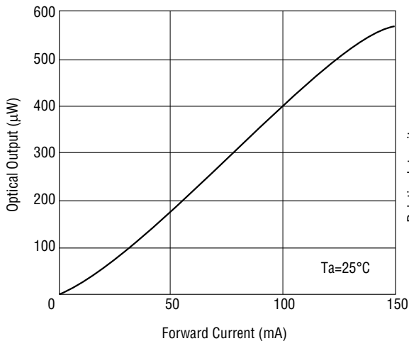
Optical Output vs. Forward Current
