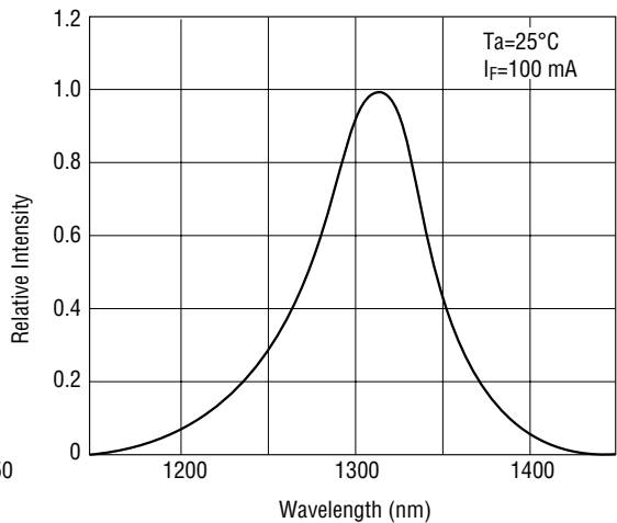
Emission Spectrum
