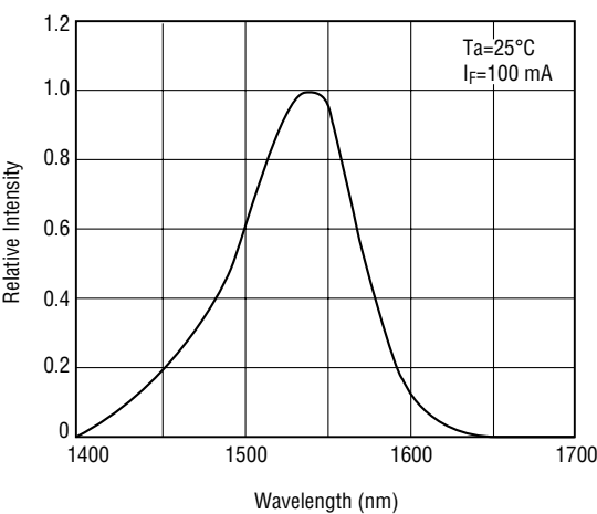
Emission Spectrum
