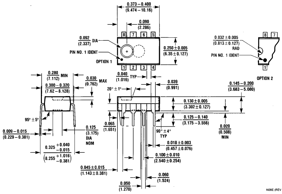
8-Lead DIP (N)
