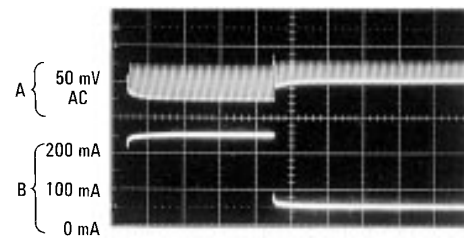
A: Output Voltage, 50 mV/div, AC Coupled B: 50 mA to 250 mA Load Pulse Horizontal Time Base: 200 \mu s/div
