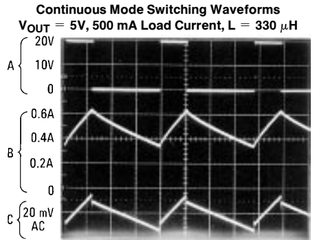
A: Output Pin Voltage, 10V/div B: Inductor Current, 0.2 A/div C: Output Ripple Voltage, 20 mV/div, AC-Coupled Horizontal Time Base: 5 \mu s/div
