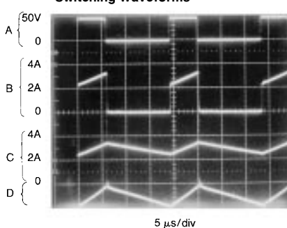
Switching Waveforms
