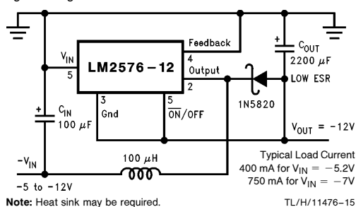
FIGURE 11. Negative Boost
