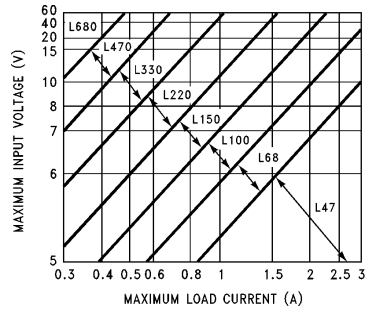
FIGURE 3. LM2576(HV)-3.3
