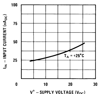
Input Current (LM2902 only)
