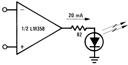
LED Driver
