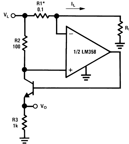
Current Monitor
