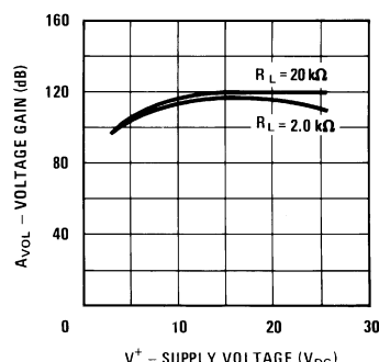
Voltage Gain (LM2902 only)
