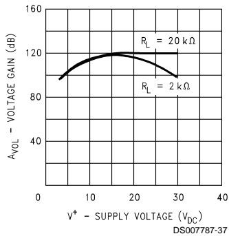
Voltage Gain
