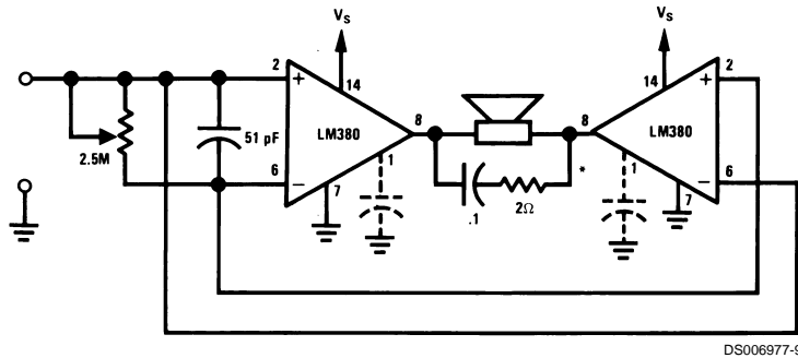
Bridge Amplifier
