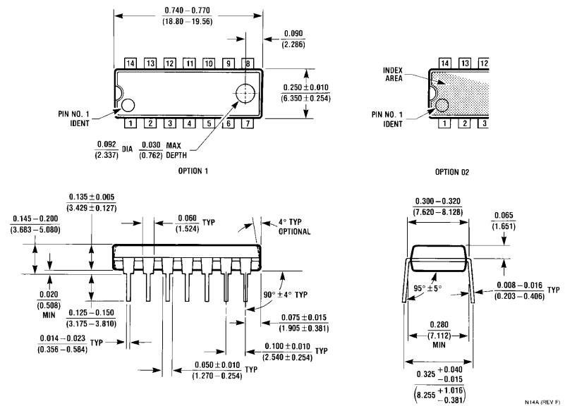
Molded Dual-In-Line Package (N) Order Number LM380N NS Package Number N14A
