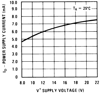
Power Supply Current vs Supply Voltage
