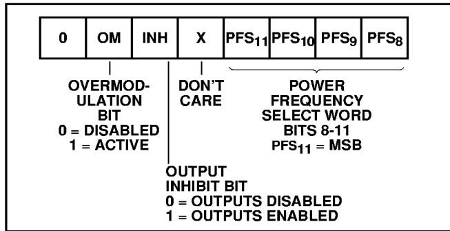
Fig. 12 Temporary register R1
