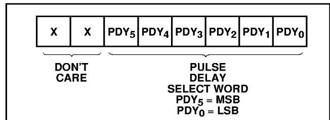
Fig. 7 Temporary register R2
