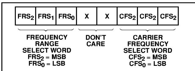
Fig. 6 Temporary register R1
