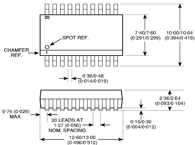
20-LEAD MINIATURE PLASTIC DIL - MP20
