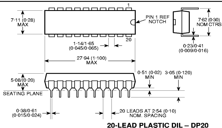
20-LEAD PLASTIC DIL - DP20
