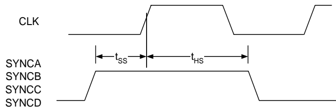
Figure 9. SYNC Timing Inputs
