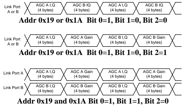
Figure 40. Link Port Data from AGC
