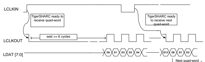
Figure 41. Link Port Data Transfer
