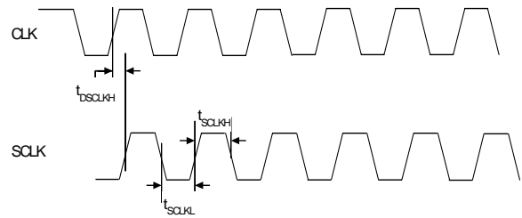
Figure 43. SCLK Switching Characteristics (Divide by 1)
