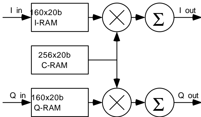
Figure 29. RAM Coefficient Filter Block Diagram
