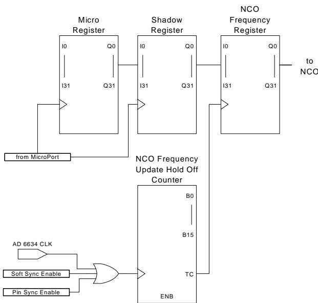
Figure 32. NCO Shadow Register and Hold Off Counter
