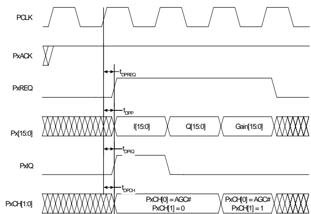
Figure 37. AGC with gain word.
