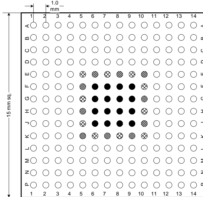
196 Lead BGA (15mm x 15mm) Top View
