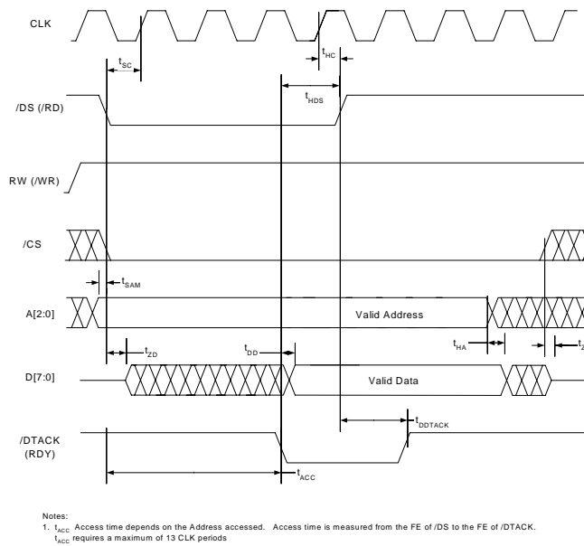
Figure 20. MNM Microport Read Timing Requirements.
