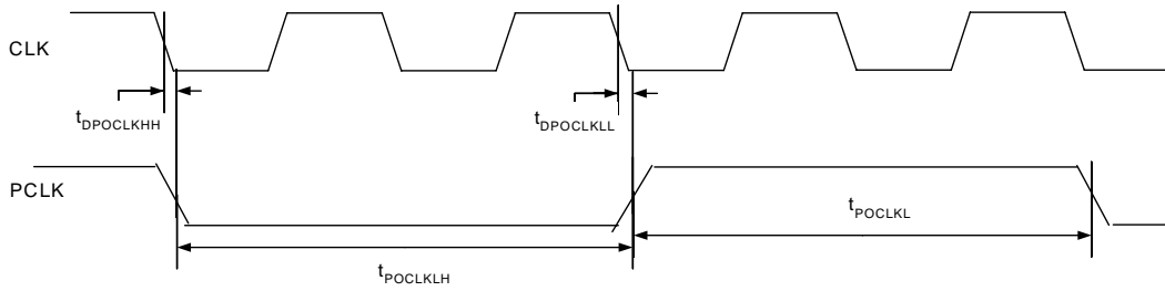
Figure 11. PCLK to CLK Switching Characteristics Divide by 2,4, or 8
