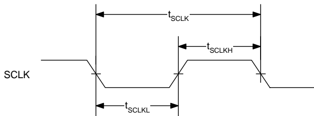
Figure 42. SCLK Timing Requirements
