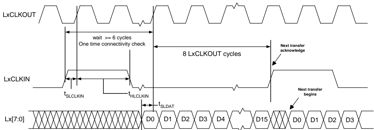
Figure 16. LxCLKIN to Lx[7:0]Data Switching Characteristics
