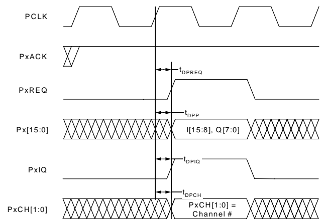
Figure 35. Channel mode 8I/8Q parallel format.
