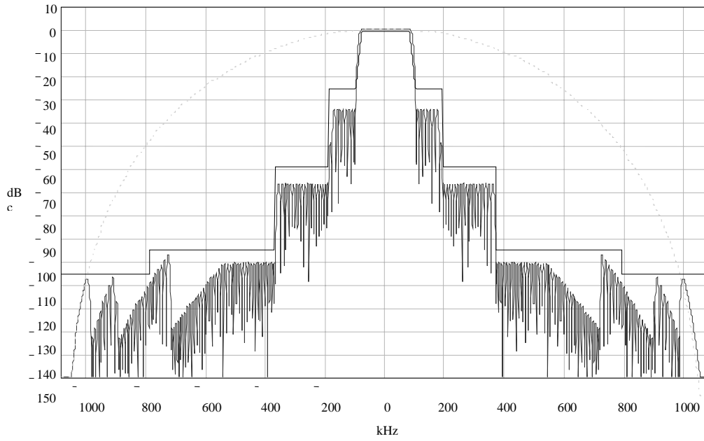
Figure 21. The filter above is based on a 65 MSPS input data rate and an output rate of 541.6666 kSPS (2 samples per symbol for EDGE). Total decimation rate is 120 distributed between the rCIC2, CIC5 and RCF.
