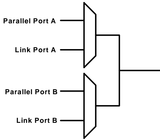
Figure 33 Output port data routing.
