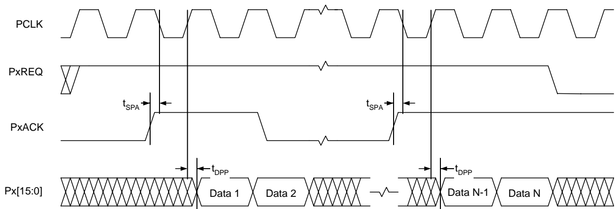
Figure 13. PxAck to PCLK Switching Characteristics
