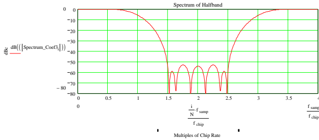
Figure 30. Interpolating Halfband Frequency Response
