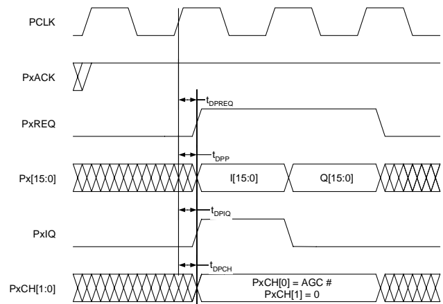
Figure 36. AGC with no gain word.
