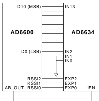
Figure 27. Typical Interconnection of the AD6600 gain-ranging ADC and the AD6634.
