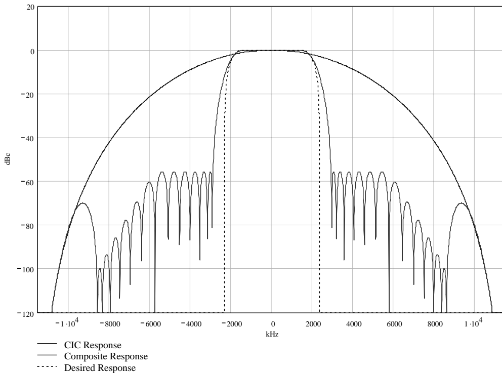
Figure 22. The filter above is designed to meet the UMTS specifications. For this configuration, the clock is set to 76.8 MSPS with 20x chip rate (3.84MCPS) and a 2x output data rate of 7.68MCPS using two channels of the AD6634.
