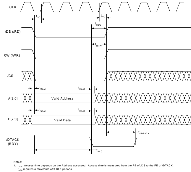
Figure 19. MNM Microport Write Timing Requirements.
