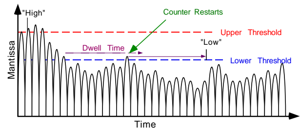
Figure 25. Threshold Settings for LI
