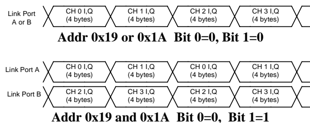
Figure 39. Link Port Data from RCF
