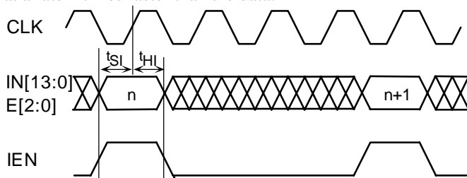
Figure 28. Fractional Rate Input Timing (4X CLK) in mode 01.
