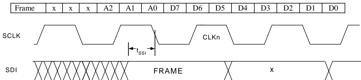
Figure 45. Serial Port Control Timing
