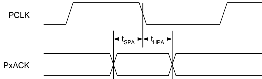
Figure 12. PxAck to PCLK Setup and Hold Characteristics
