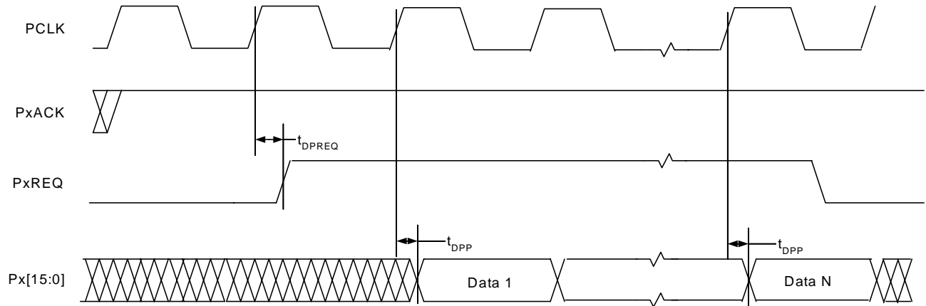
Figure 14. PxrEQ to PCLK Switching Characteristics
