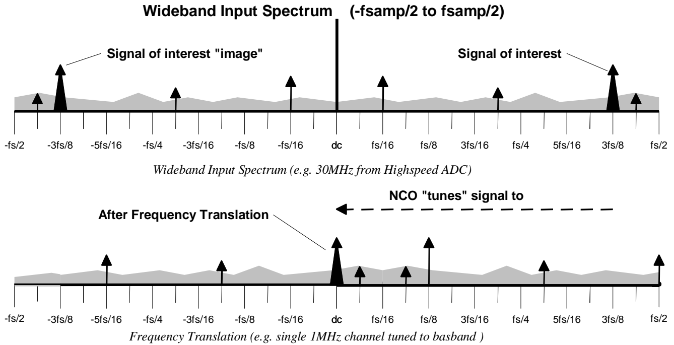
Figure 2a. AD6634 Frequency Translation of Wideband Input Spectrum
