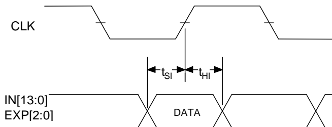
Figure 23. Input Data Timing Requirements
