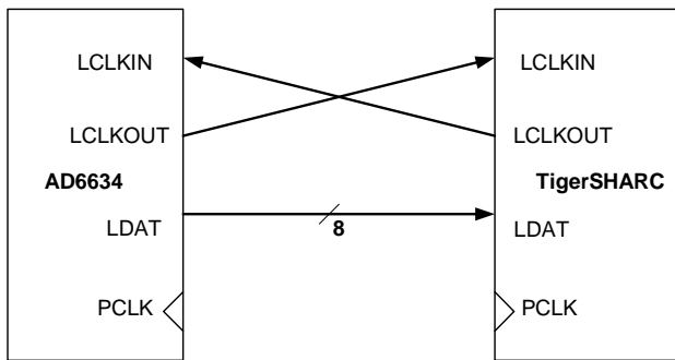
Figure 38. Link Port Connection Between AD6634 and TigerSHARC
