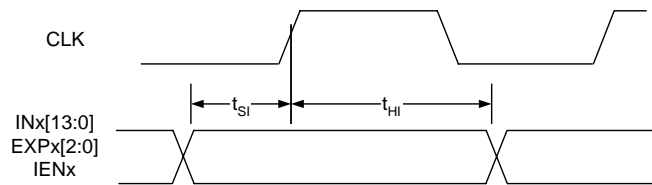
Figure 8. Input Timing for A and B Channels
