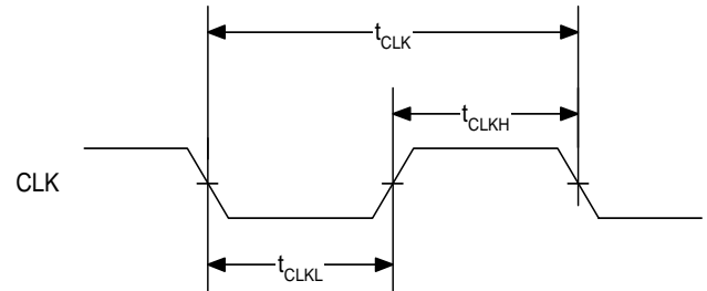
Figure 24. CLK Timing Requirements
