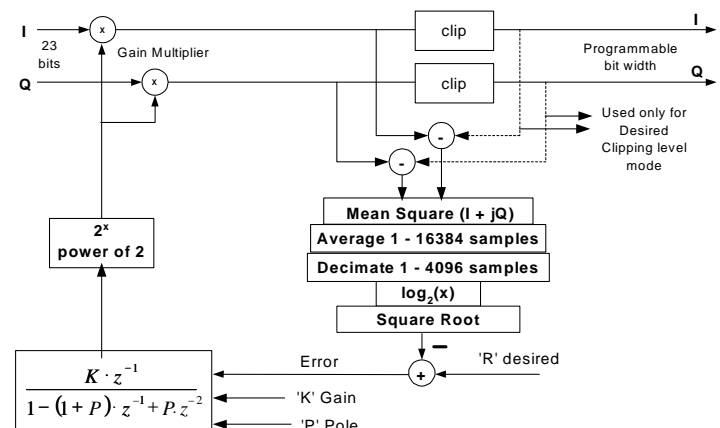
Figure 31: Conceptual Block Diagram of the AGC
