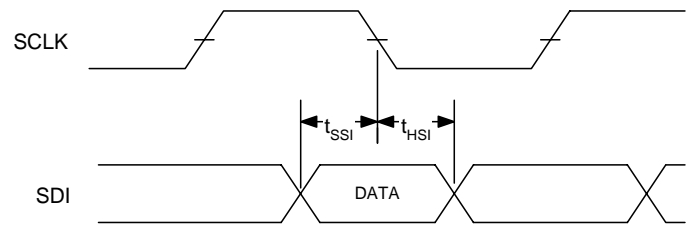
Figure 44. Serial Input Data Timing Requirements
