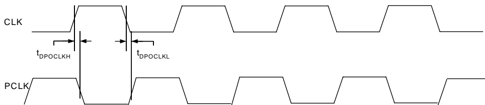
Figure 10. PCLK to CLK Switching Characteristics Divide by 1
