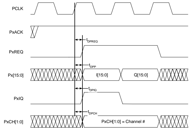
Figure 34. Channel mode interleaved format.
