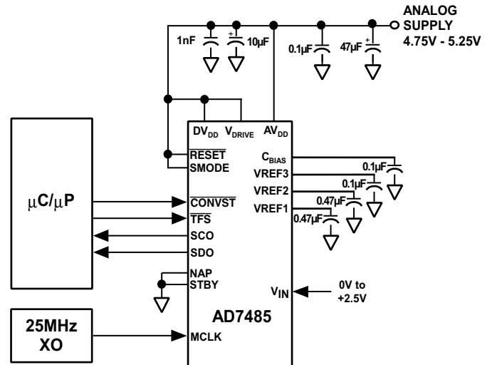
Figure 9. AD7485 Typical Connection Diagram
