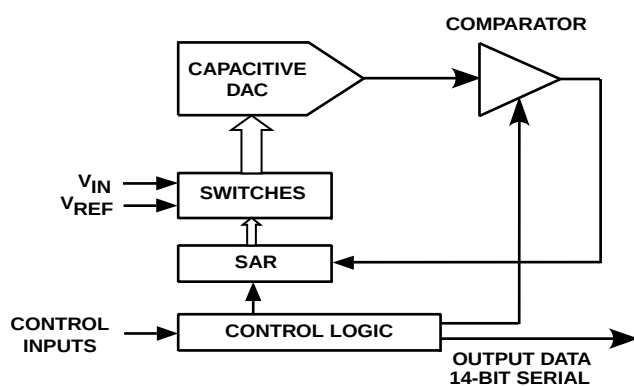
Figure 1. Simplified Block Diagram of AD7485
