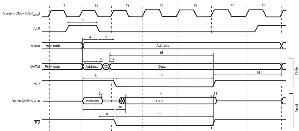
Figure 119. External Memory Timing (SRWn1 = 1, SRWn0 = 1) (1)
