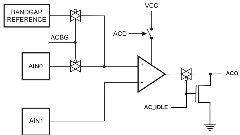
Figure 91. Analog Comparator
