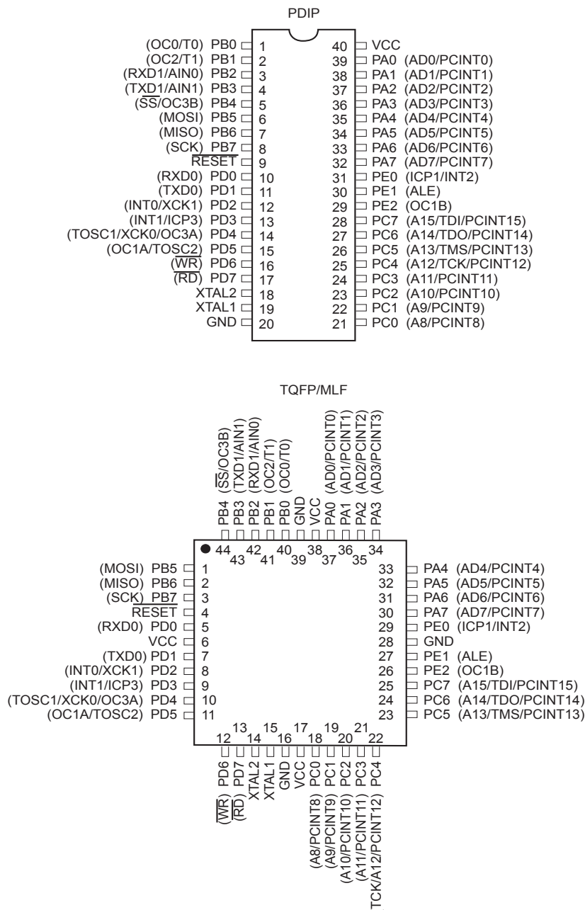
Figure 1. Pinout ATmega162
