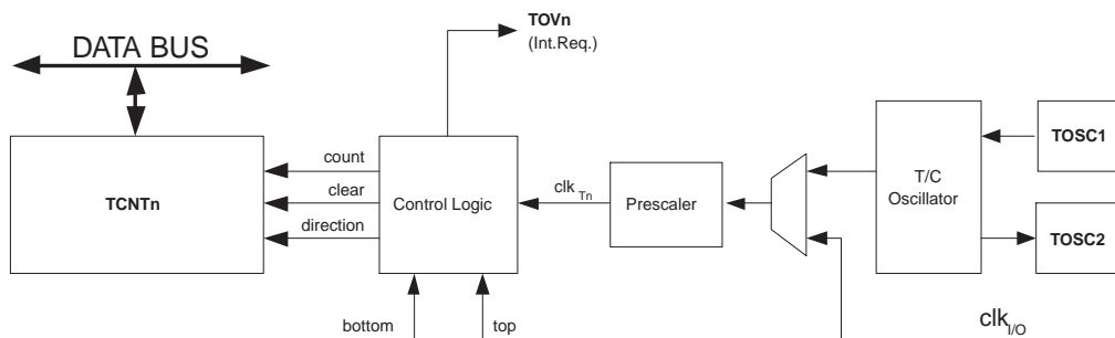
Figure 60. Counter Unit Block Diagram
