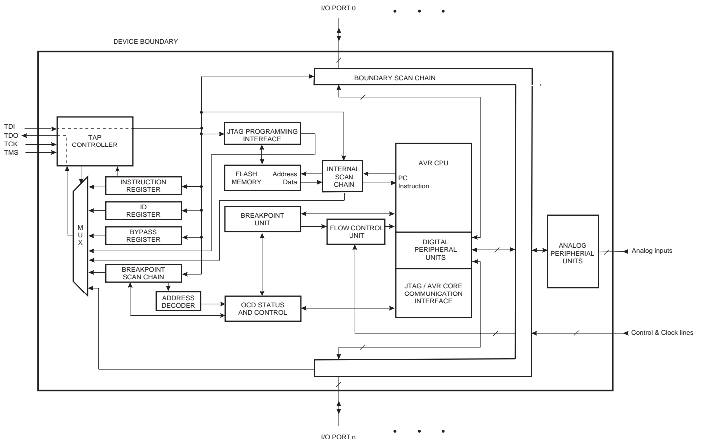
Figure 83. Block Diagram
