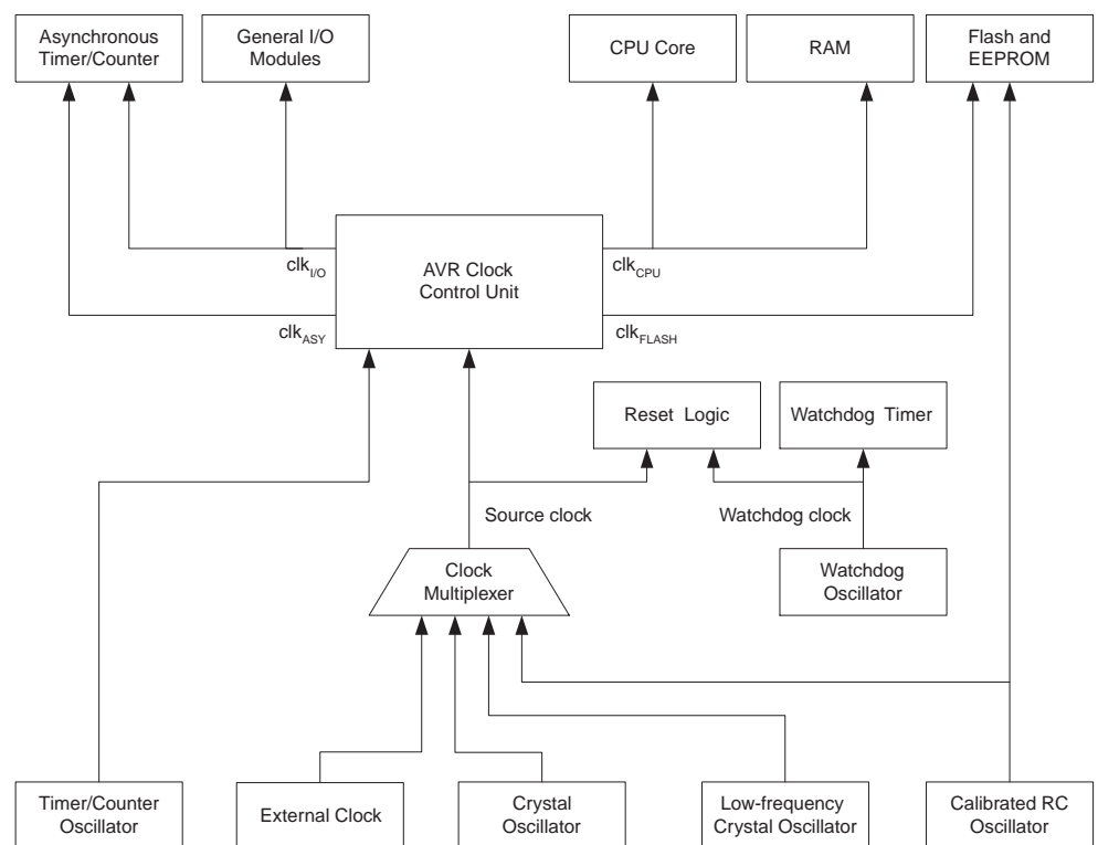
Figure 18. Clock Distribution
