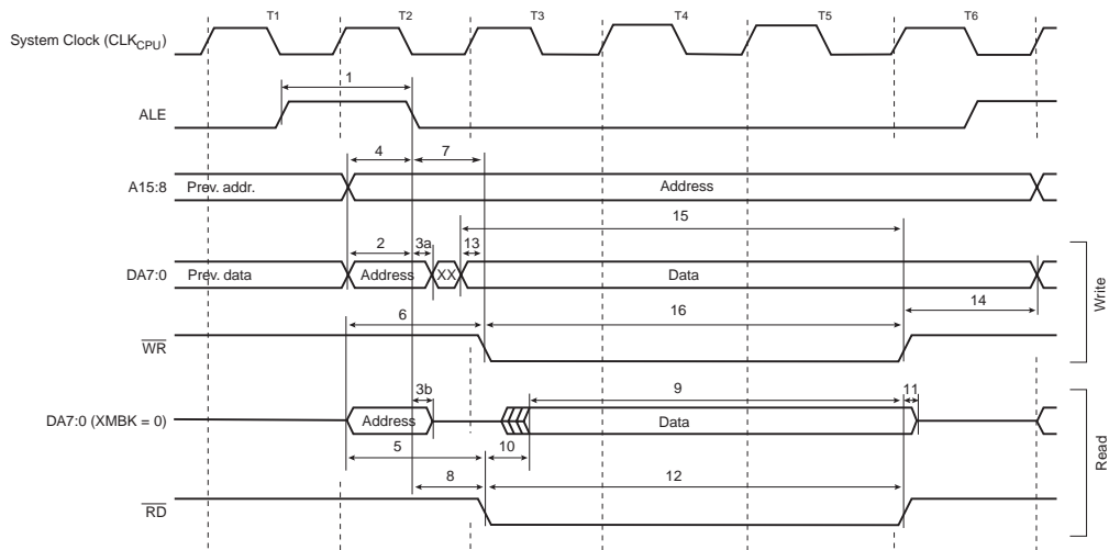
Figure 118. External Memory Timing (SRWn1 = 1, SRWn0 = 0)
