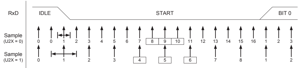
Figure 79. Start Bit Sampling
