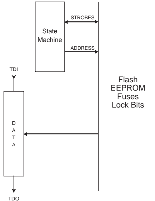
Figure 112. Virtual Flash Page Read Register
