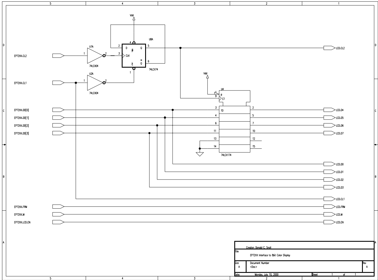
Figure 1. EP72xx Interface to 8-Bit Color Display
