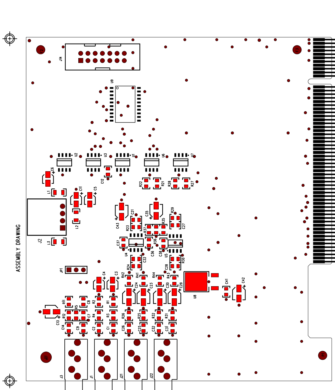
Figure 5. Assembly Drawing
