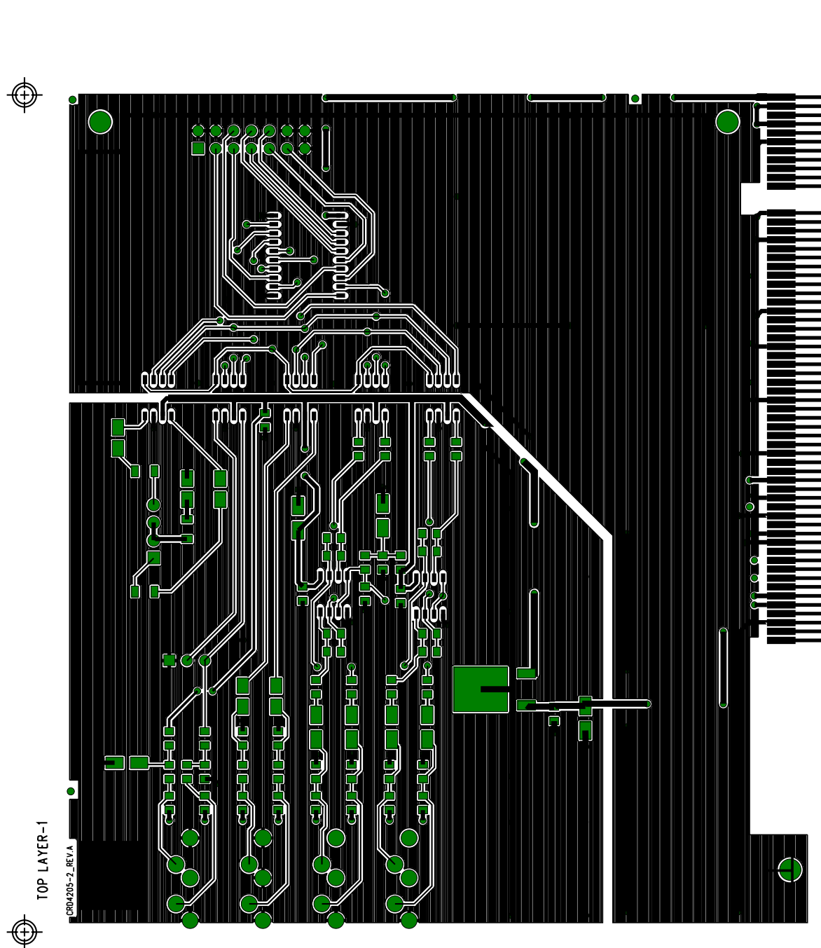
Figure 7. Top Layer
