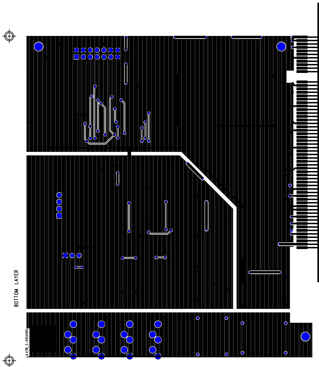
Figure 8. Bottom Layer
