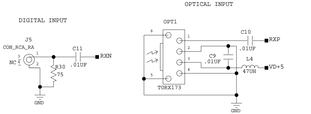
Figure 6. Digital Audio Inputs
