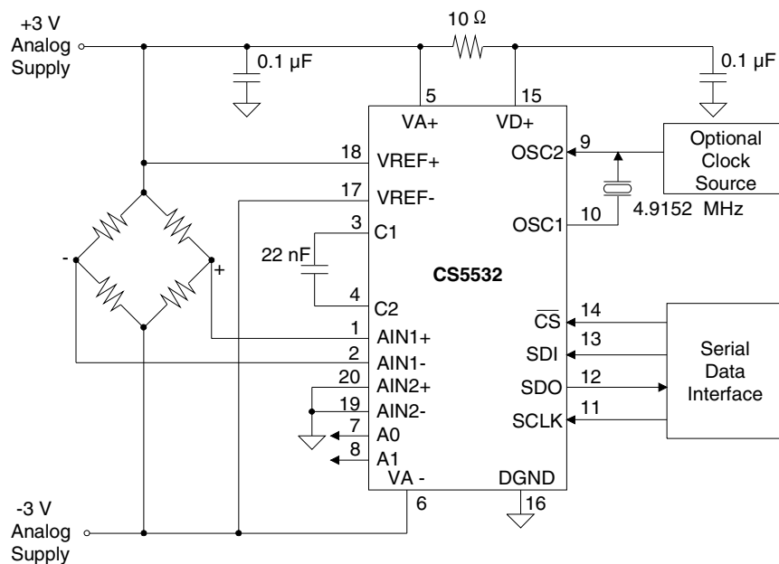
Figure 22. CS5532 Configured with \pm 3 V Analog Supplies
