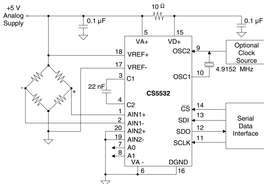
Figure 20. CS5532 Configured with a Single +5 V Supply
