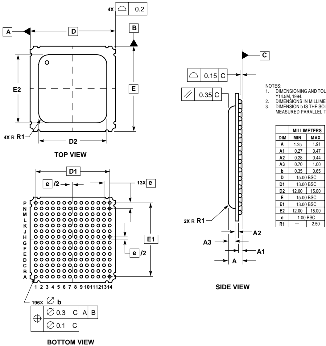
Figure 3-3 DSP56307 Mechanical Information, 196-pin PBGA Package
