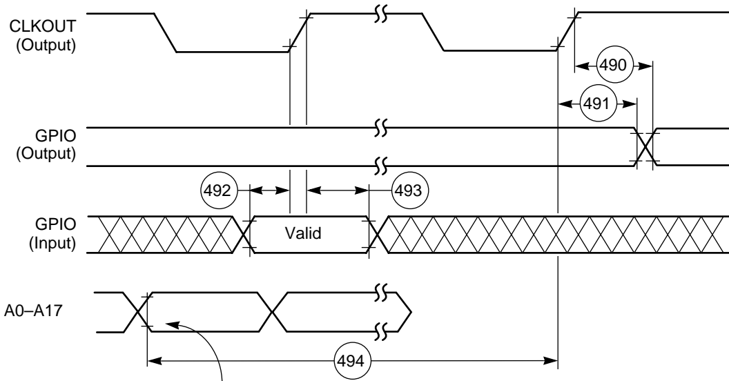
Figure 2-40 GPIO Timing
