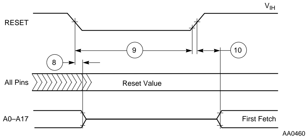
Figure 2-3 Reset Timing
