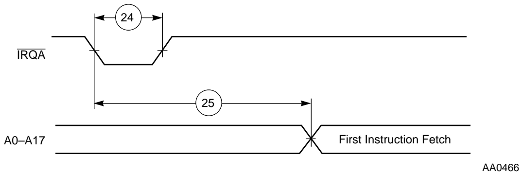
Figure 2-9 Recovery from Stop State Using \overline{\text{IRQA}}
