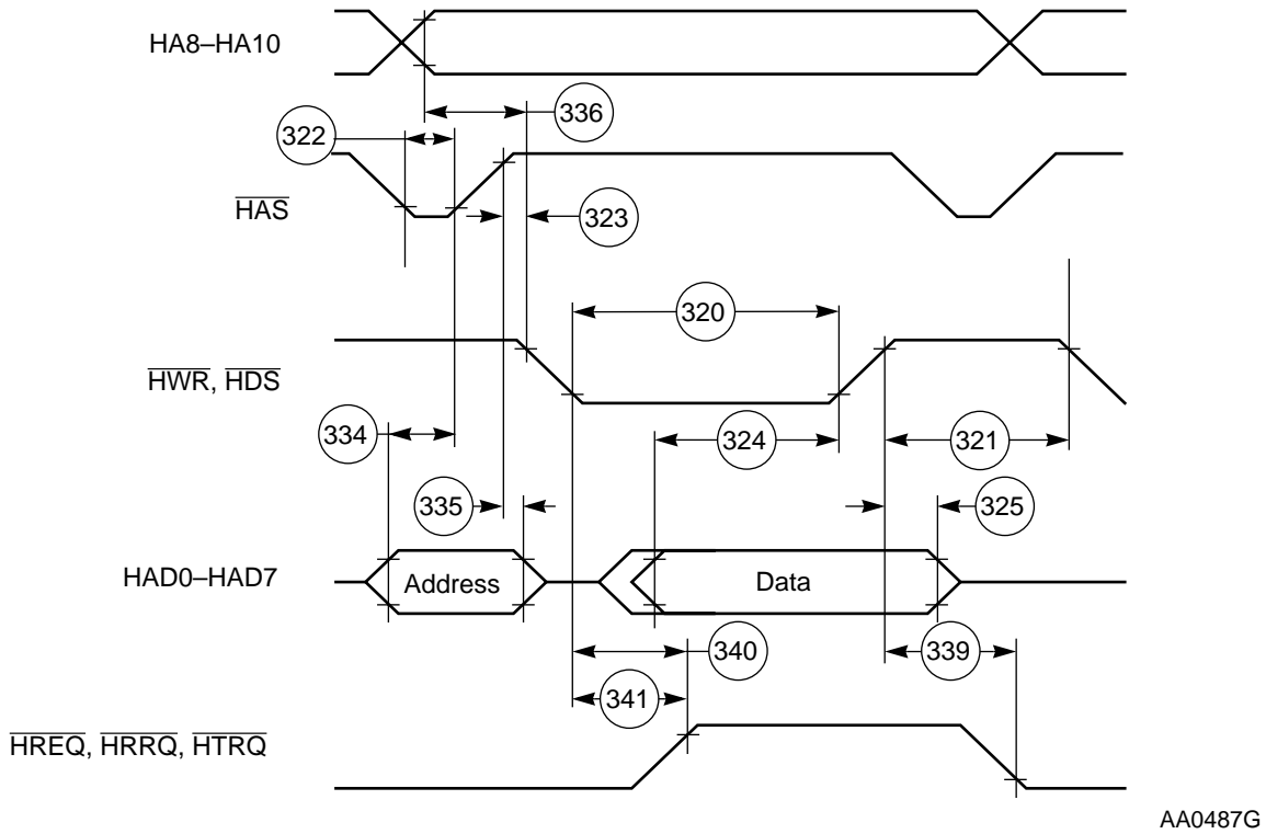
Figure 2-32 Write Timing Diagram, Multiplexed Bus
