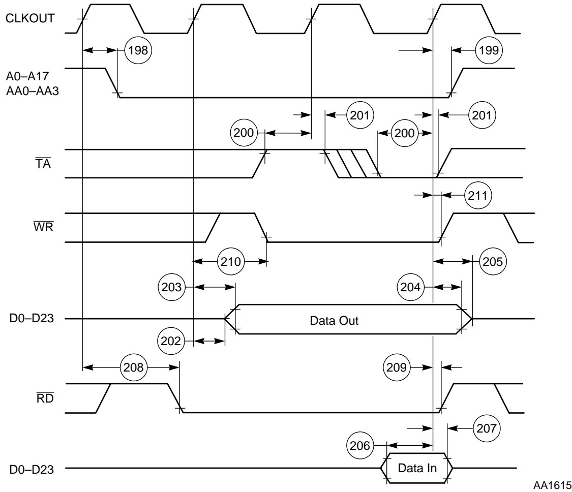
Figure 2-22 Synchronous Bus Timings, SRAM, 2 or More WS, TA Controlled
