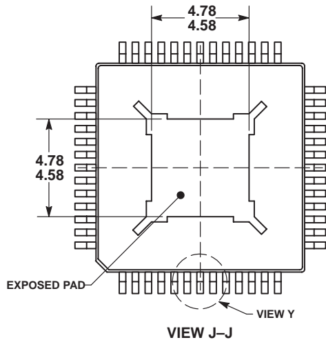
VIEW J-J
