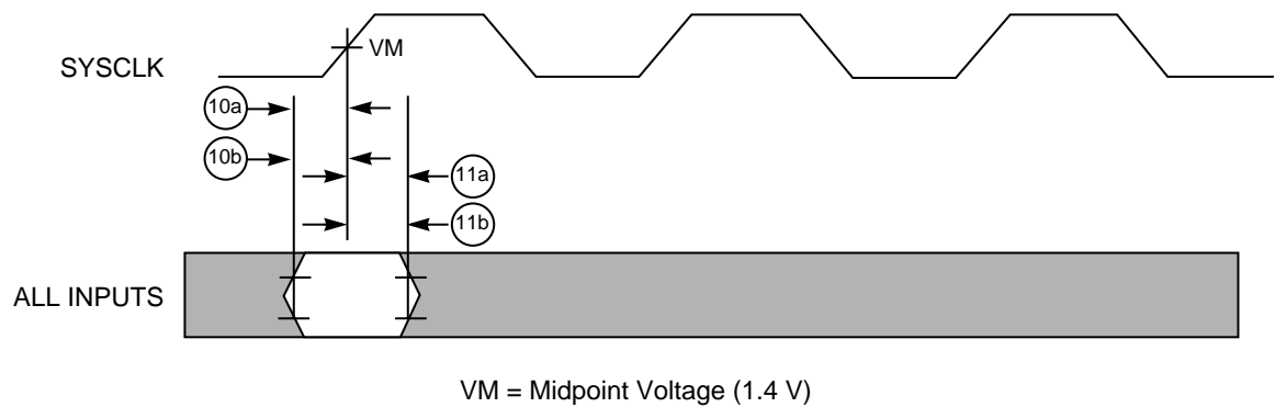
Figure 2. Input Timing Diagram
