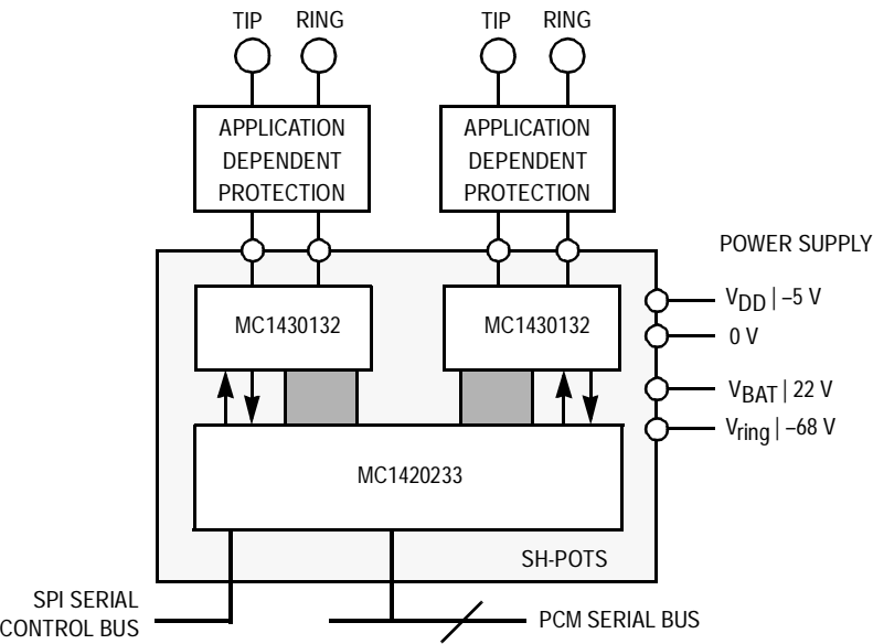
Figure 1. Block Diagram
