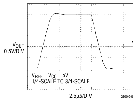
Large-Signal Settling
