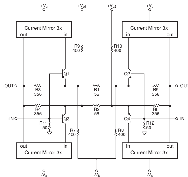
Figure 1: KH600 Simplified Schematic
