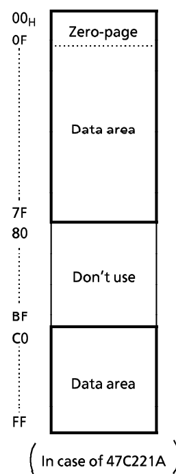
Figure 1-2. RAM addressing ( In case of 47C221A )
