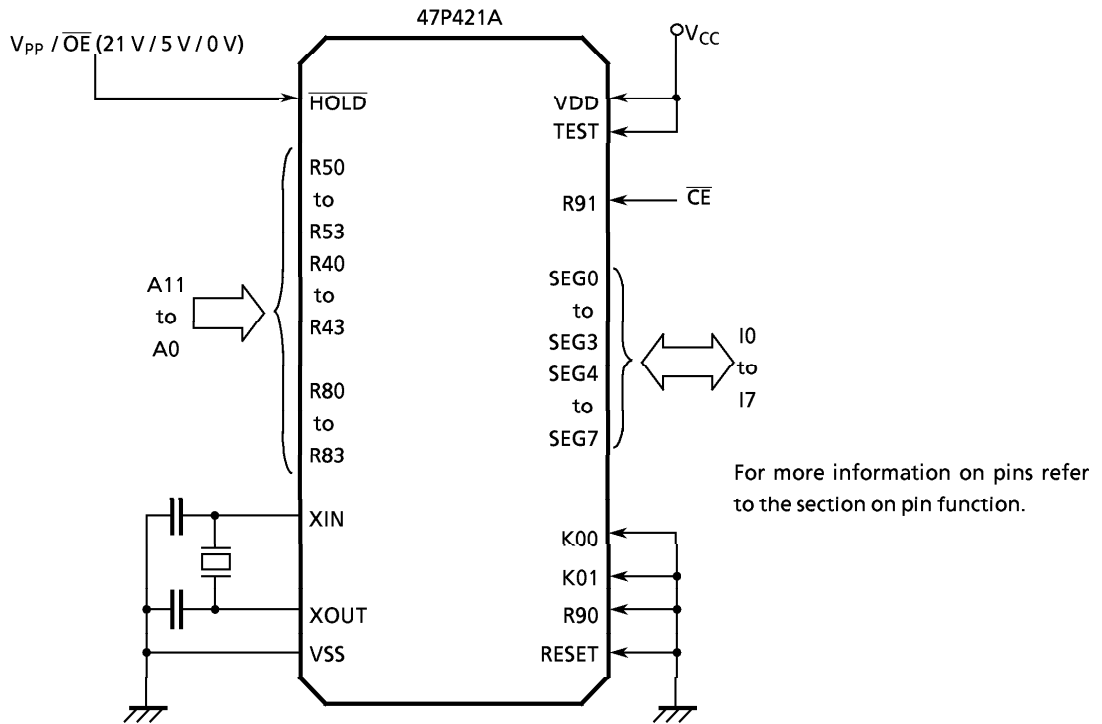
Figure 1-4. Setting for PROM mode
