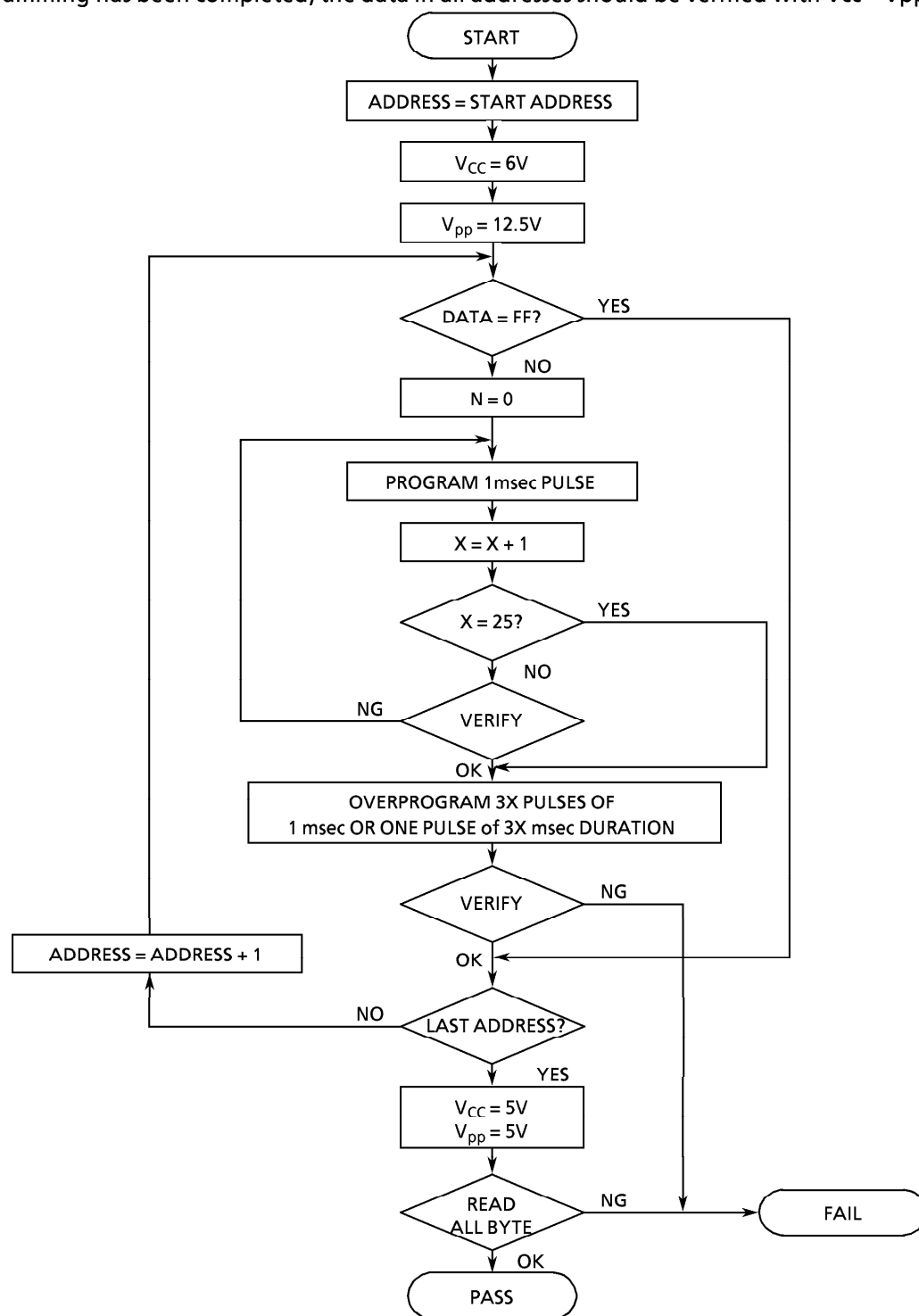
Figure1-4. FLOW CHART
