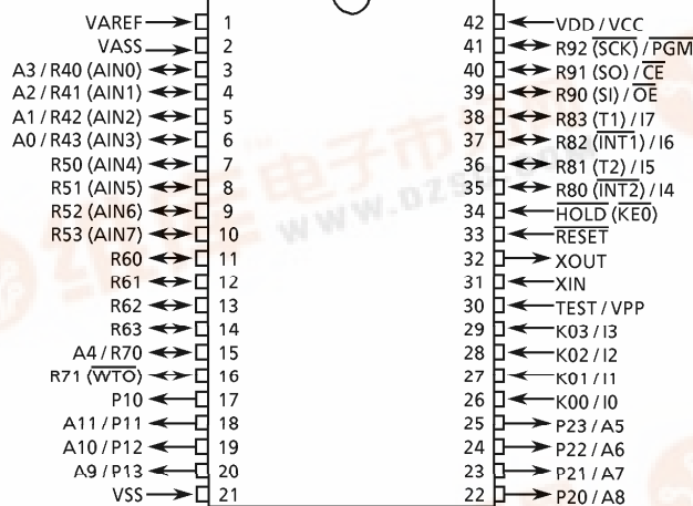
SDIP42-P-600-1.78
