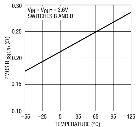
PMOS R_{DS(ON)}
