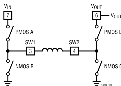
Figure 1. Simplified Diagram of Output Switches
