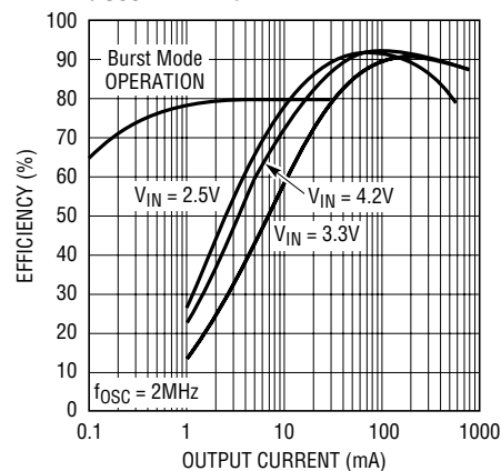
Li-Ion to 3.3V Efficiency ( f_{osc} = 2MHz )
