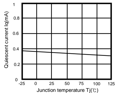
Figure 6. Quiescent Current vs. Temperature( T_j )
