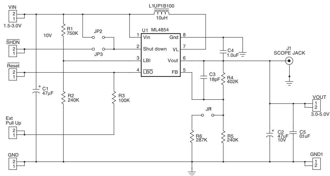
Figure 1. Test Circuit
