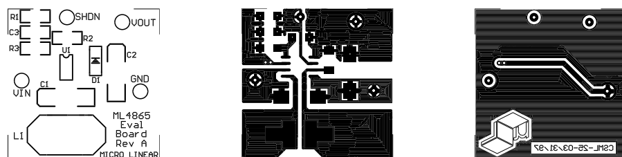
Figure 8. Sample ML4865 Layout
