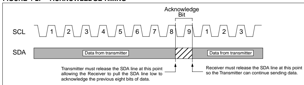
FIGURE 4-2: ACKNOWLEDGE TIMING
