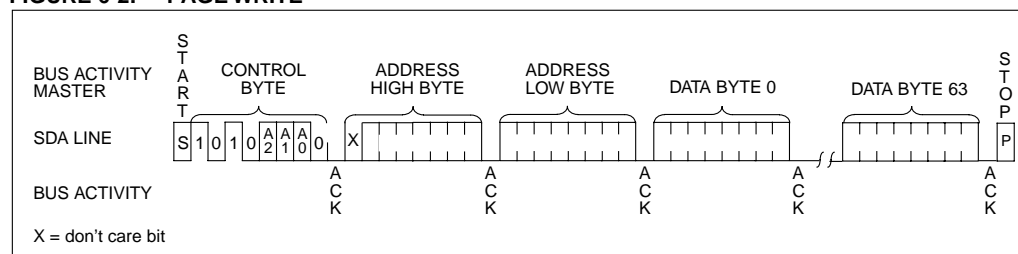
FIGURE 6-2: PAGE WRITE
