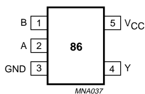
Fig.1 Pin configuration.
