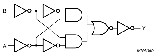
Fig.4 Logic diagram.
