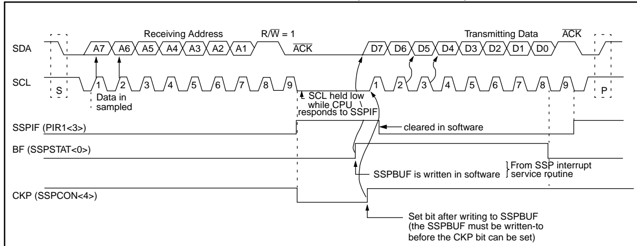
FIGURE 8-6: I 2 C WAVEFORMS FOR TRANSMISSION (7-BIT ADDRESS)
