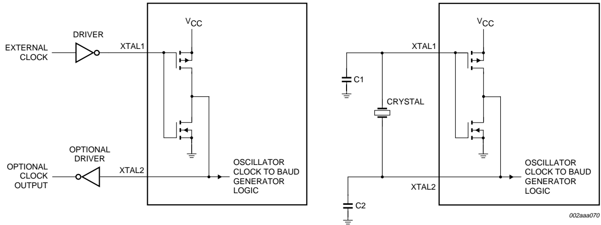
Fig 12. Typical crystal clock circuits.
