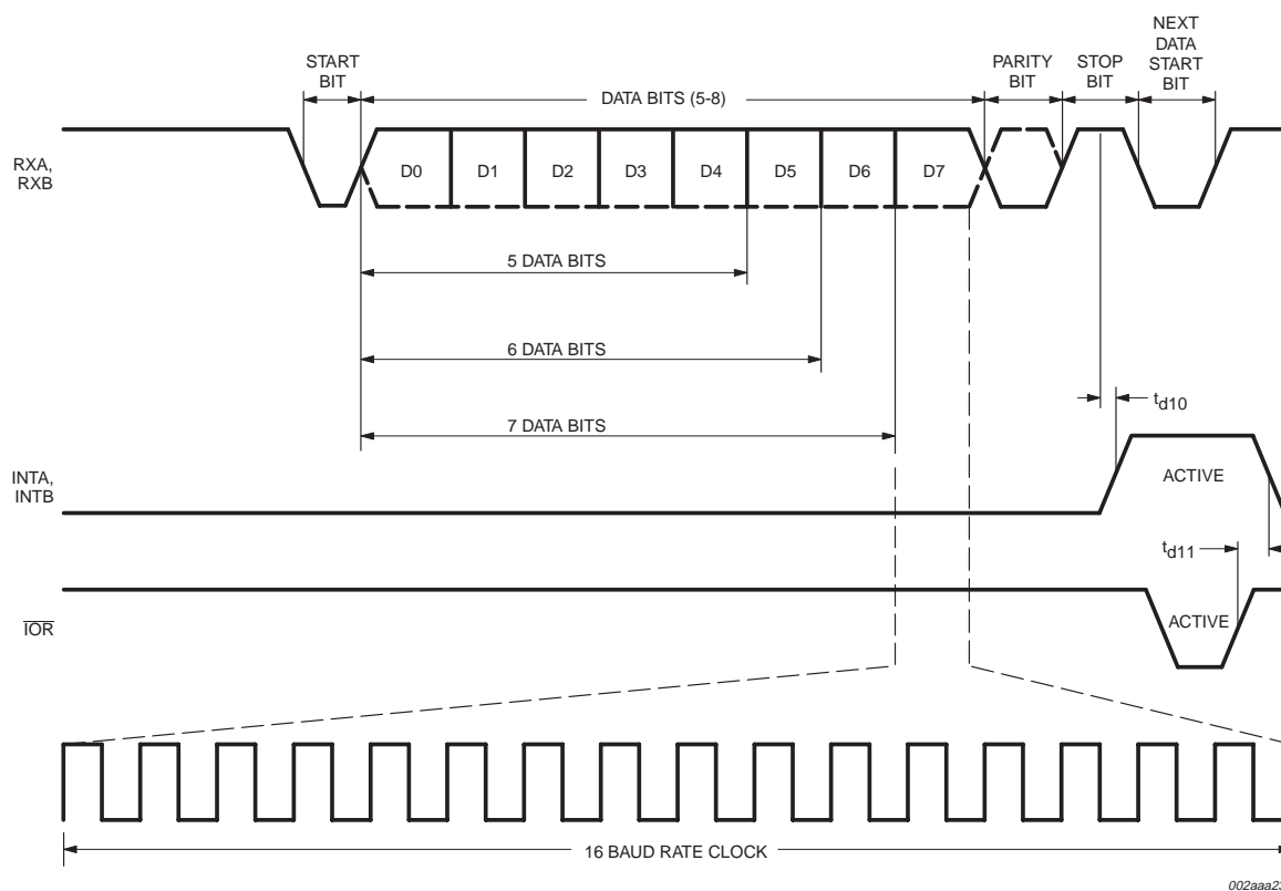
Fig 17. Receive timing.
