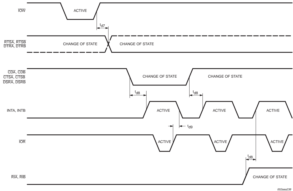
Fig 16. Modem input/output timing.
