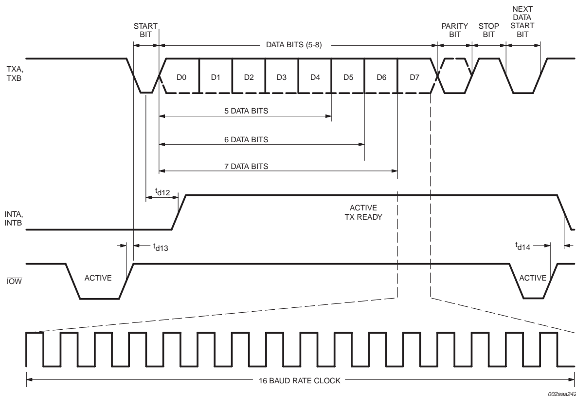
Fig 20. Transmit timing.
